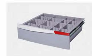
Two middle drawers panel height 120mm inner size: 508×358×108mm
