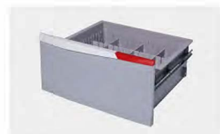
One big drawer panel height 238mm inner size: 508×358×223mm
