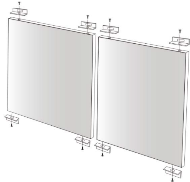
Installation Diagram
