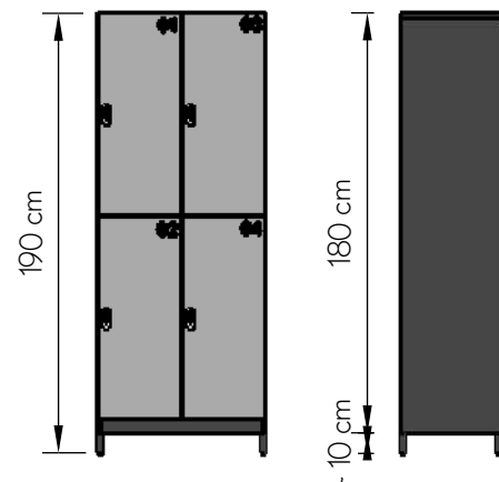
LOCKER ON ADJUSTABLE LEGS
