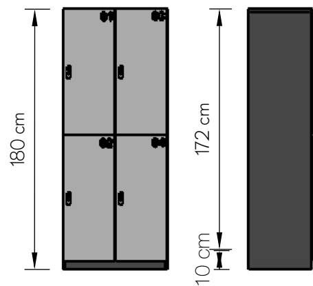
LOCKER ON A SOCLE
